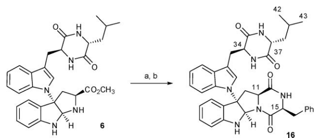
Scheme 3 Reagents and conditions: (a) N -Fmoc-L-phenylalanine (1.1 equiv.), HATU (1.1 equiv.), \text{Et}_3\text{N} (2.2 equiv.), DMF, 0 to 25^\circ\text{C} . (b) \text{Et}_2\text{NH} (55 equiv.), MeOH, 25^\circ\text{C} , 56% combined.
