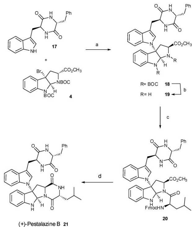
Scheme 4 Reagents and conditions: (a) \text{KOtBu} (2.0 equiv.), \text{CH}_3\text{CN} , 12^\circ\text{C} , 30%. (b) TMSI (2.2 equiv.), \text{CH}_3\text{CN} , 0^\circ\text{C} , 85%. (c) 1) N -Fmoc-D-leucine (1.1 equiv.), HATU (1.1 equiv.), \text{Et}_3\text{N} (2.2 equiv.), DMF, 0 to 25^\circ\text{C} . 2) \text{Et}_2\text{NH} (55 equiv.), MeOH, 25^\circ\text{C} , 57% combined.
